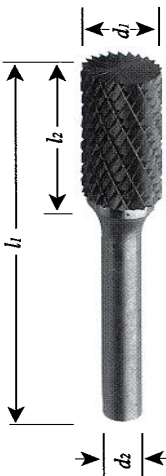
Cylinder Shape - End Cut (SB Series)
